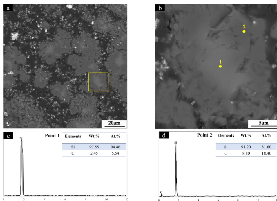
Fig. 5. a,b) SEM-BSE micrographs and c,d) EDS analysis of various points of the C/C-SiC-HfC composite
